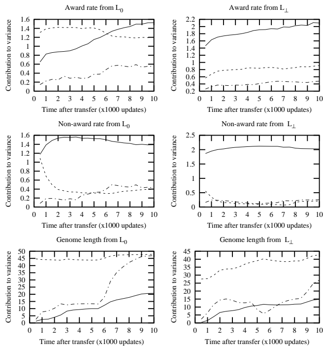
Figure 5: Contributions of adaptation (lines), history (dashes) and chance (dash-dotted) to variance in award rate (top), non-award rate (middle) and genome length (bottom) in populations transferred from landscape L_0 (left) and L_{\perp} (right) to landscape L_T .
